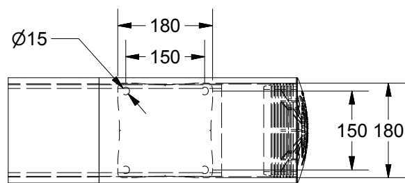
DETAIL A SCALE 1/10 END POST
