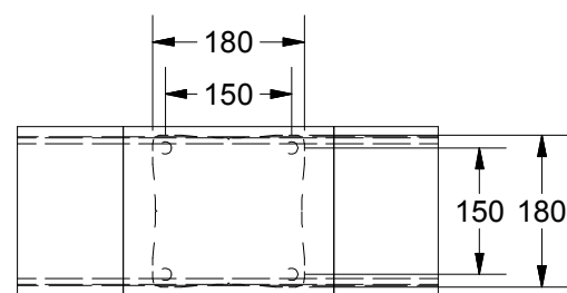
DETAIL B SCALE 1/10 MID POST
